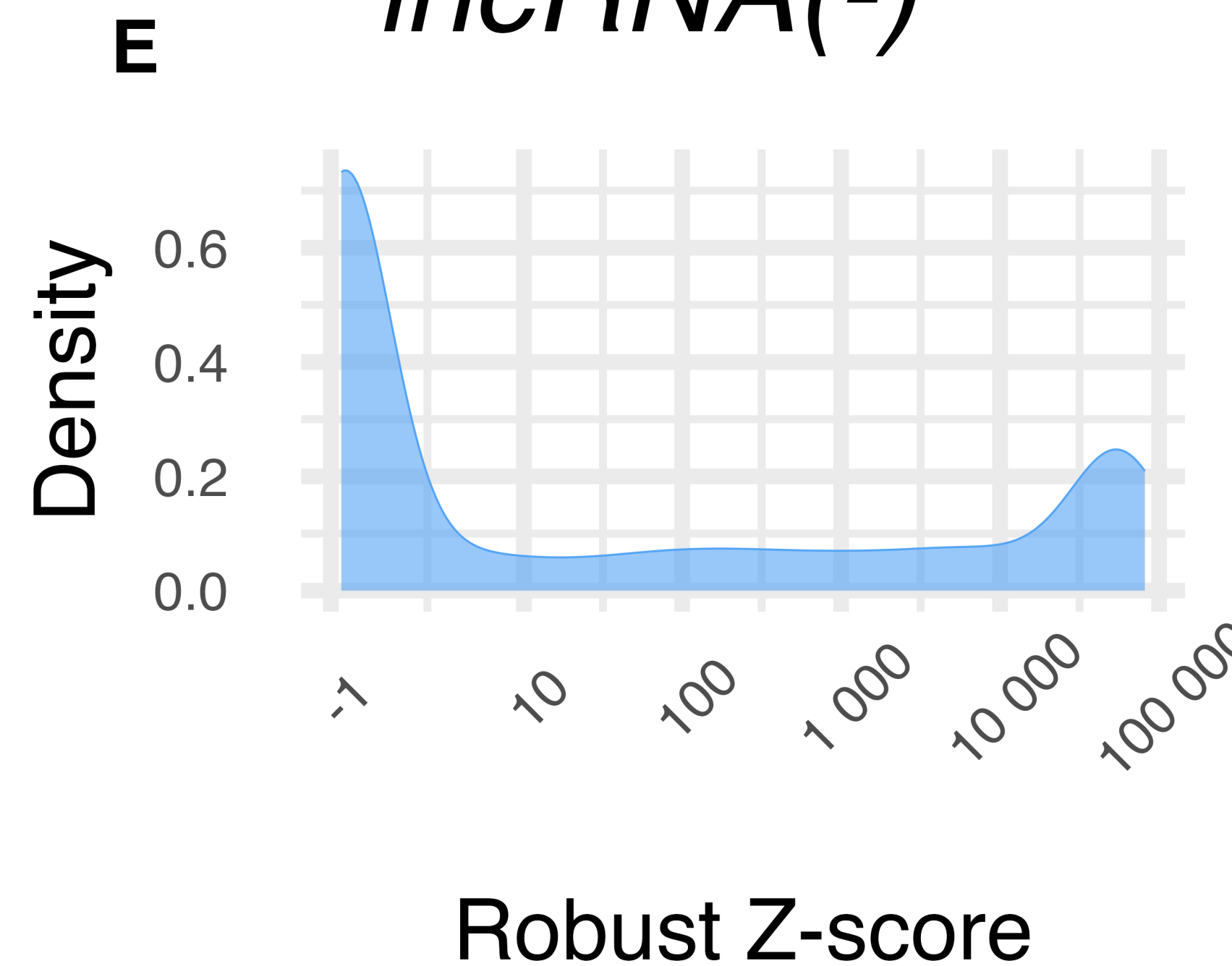
Supplementary Figure S10. lncRNA copies robust z-scores distributions in log scale. A-C) Histogram, Density and Boxplot for lncRNA(+), D-F) Histogram, Density and Boxplot for lncRNA(-). The positive dataset shows log (robust z-scores) centered around 0.1 which also applies for the negative set. It is important however to highlight that there is greater spread for negative set compared to the positive set, which indicates the two dataset come from different distributions
