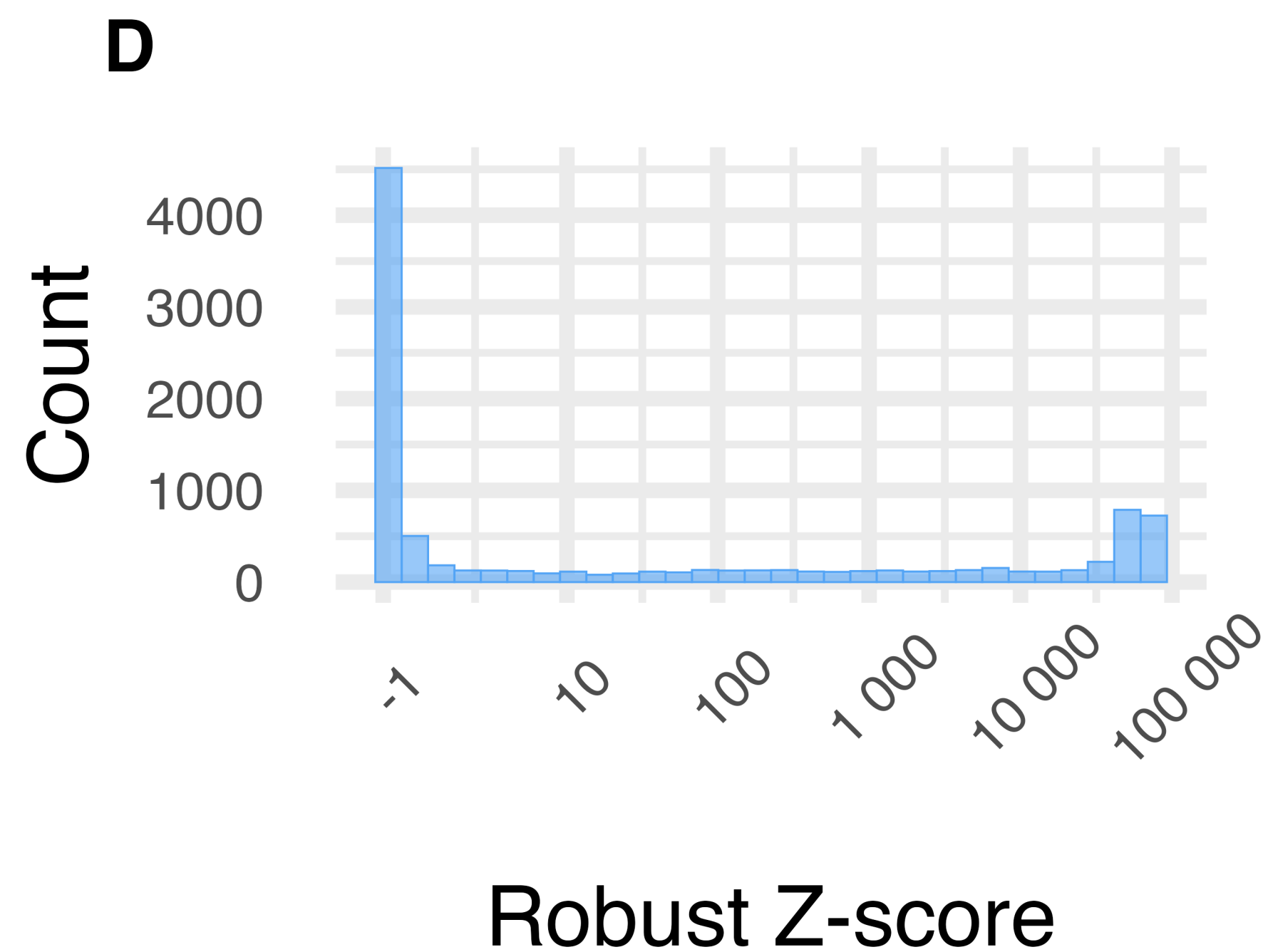
Supplementary Figure S10. lncRNA copies robust z-scores distributions in log scale. A-C) Histogram, Density and Boxplot for lncRNA(+), D-F) Histogram, Density and Boxplot for lncRNA(-). The positive dataset shows log (robust z-scores) centered around 0.1 which also applies for the negative set. It is important however to highlight that there is greater spread for negative set compared to the positive set, which indicates the two dataset come from different distributions
